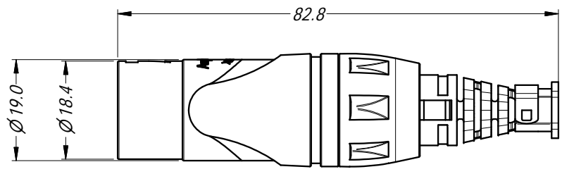
SMALL CABLE CLAMP
